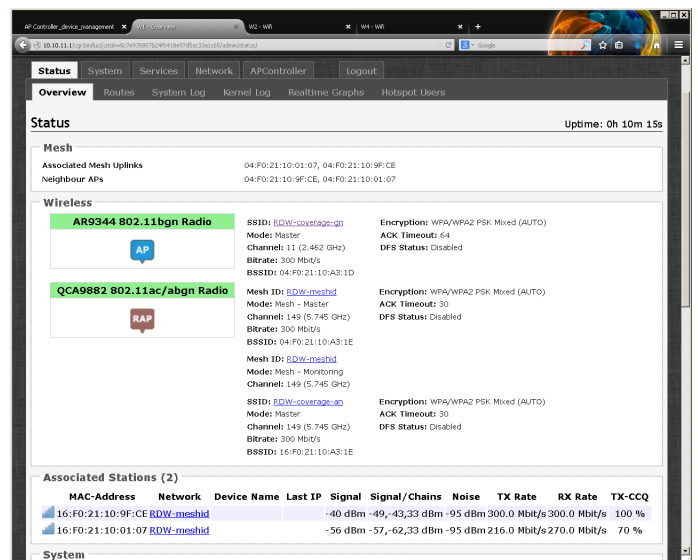
Figure 58: The Status > Overview page of an RAP.
