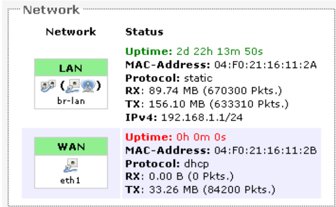
Figure 9: Network summary.
