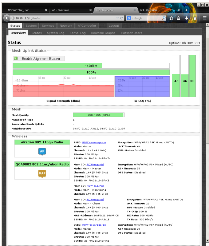
Figure 61: The Status > Overview page of an MAP.
