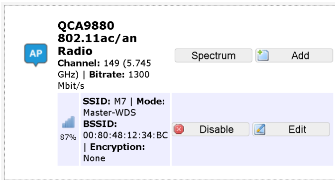
Figure 51: The first router is set to the AP WDS mode.
