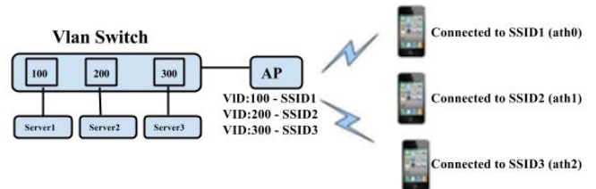
Figure 71: Clients with different SSIDs to connect different servers.
