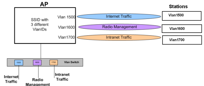
Figure 70: AP connected to 3 stations with different VLAN IDs.
